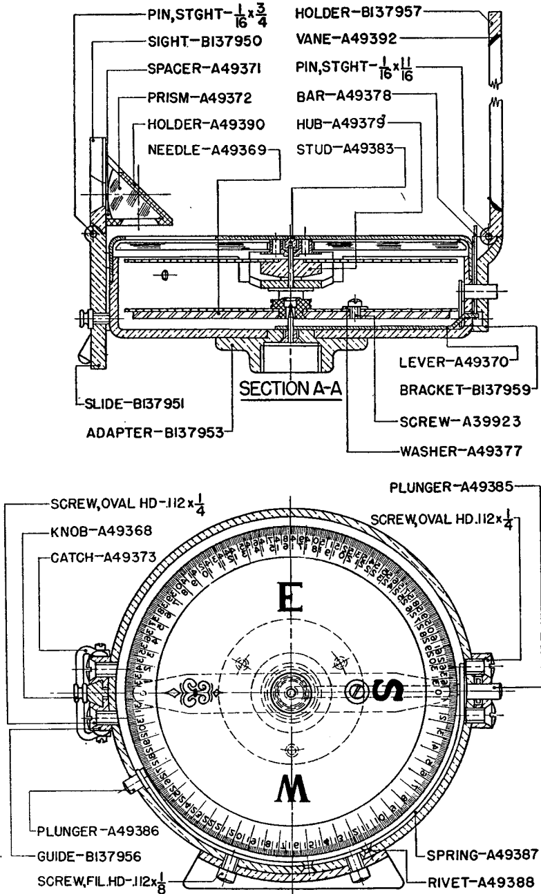
FIGURE 2.—Prismatic compass, M1918—sectional views—Continued.
